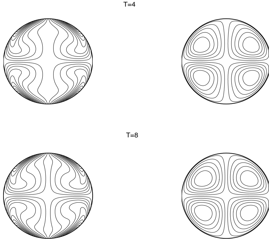
Figure 1: Vorticity contours (left) and streamlines (right) of the moving wall problem with Re = 100 .
