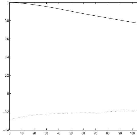
Figure 5: Time evolution of the peak vorticity for the tripole formation. '—': peak positive vorticity; '· ·': peak negative vorticity.
