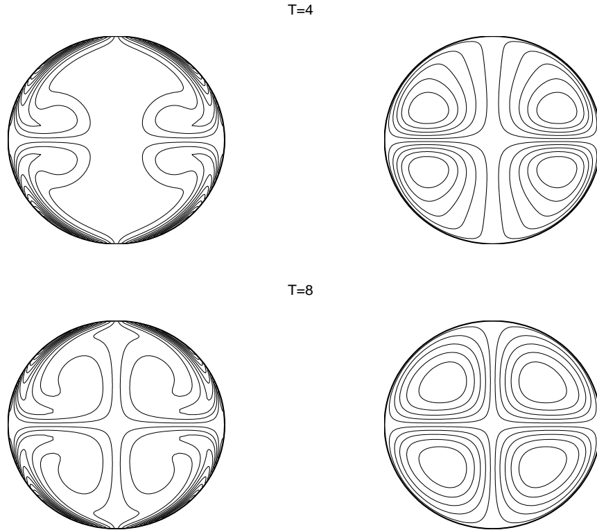
Figure 2: Vorticity contours (left) and streamlines (right) of the moving wall problem with Re = 300 .
