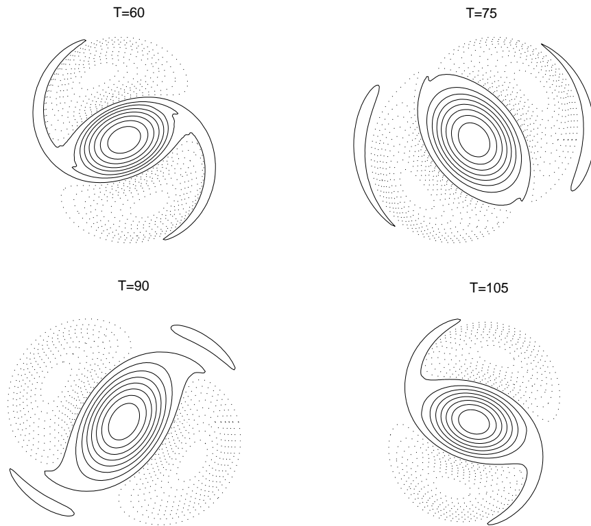
Figure 4: Vorticity contour plots of the tripole formation from T = 60 to T = 105 . '-' positive values, '.' negative values.
