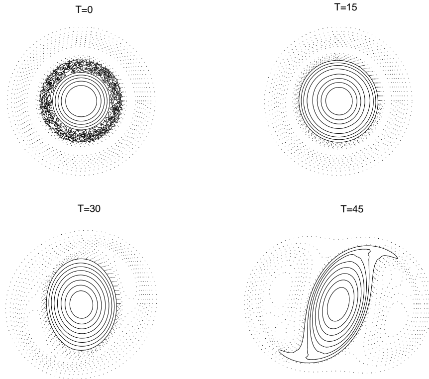
Figure 3: Vorticity contour plots of the tripole formation from T = 0 to T = 45 . '-' positive values, '.' negative values.
